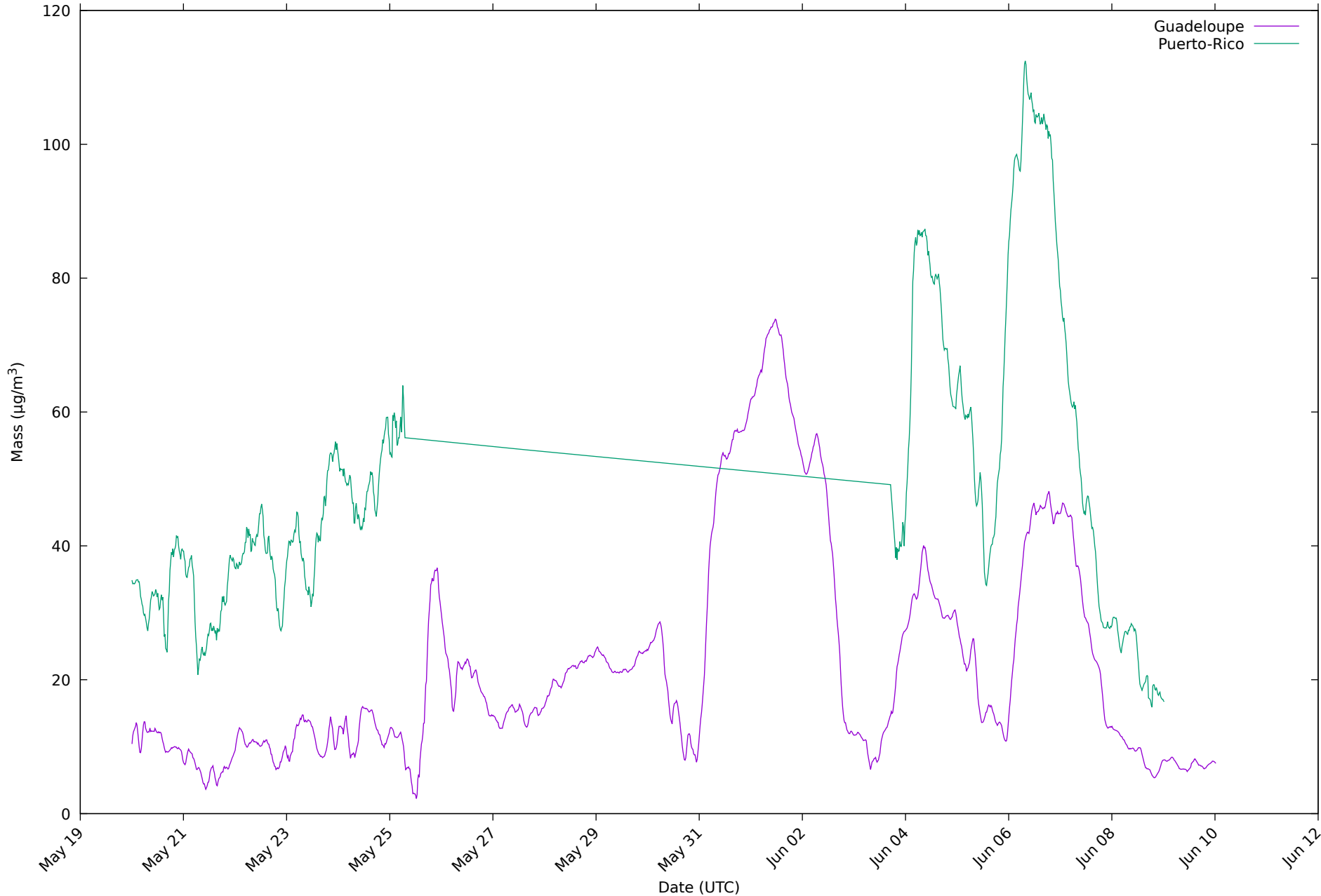
PM10 in Caribbeans ends on Jun 10, 2026
